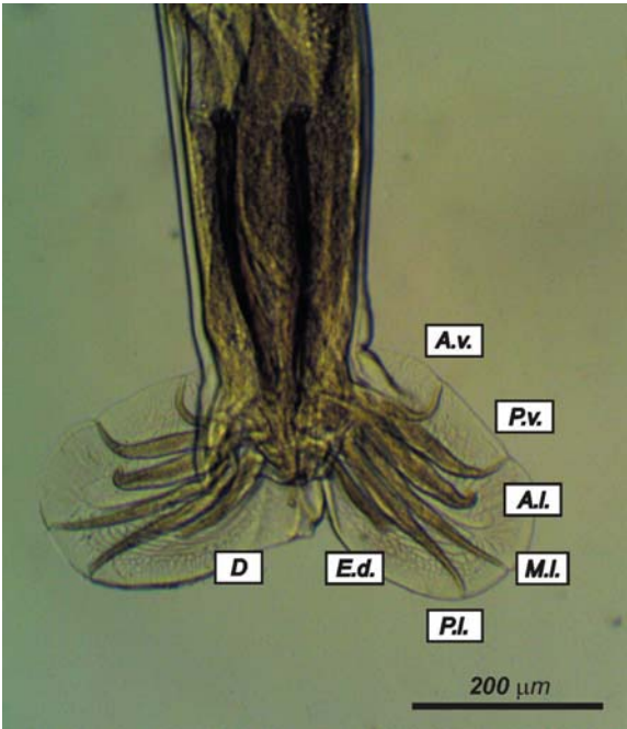
Fig. 2. Caudal end of ♂ Amidostomum anseris : A.v. — anteroventral ray; P.v. — posteroventral ray; A.l. — anterolateral ray; M.l. — mediolateral ray; P.l. — posterolateral ray; E.d. — external and dorsal ray; D — dorsal ray.
